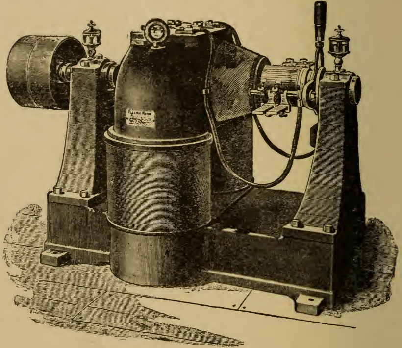
Fig. 17. STATIONARY MOTOR.
